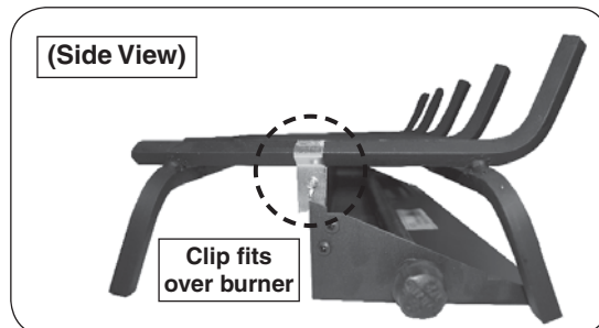
Fig. 12-3 Grate placement detail
