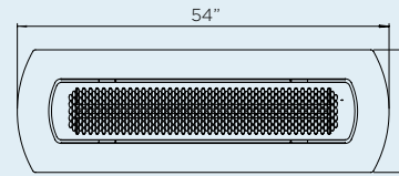
CEILING RECESS FRAME 2000W & 4000W
