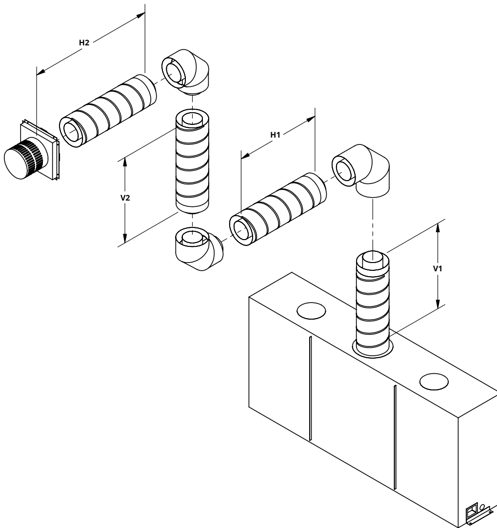
Figure 8.f Horizontal Termination - 3 Elbows
